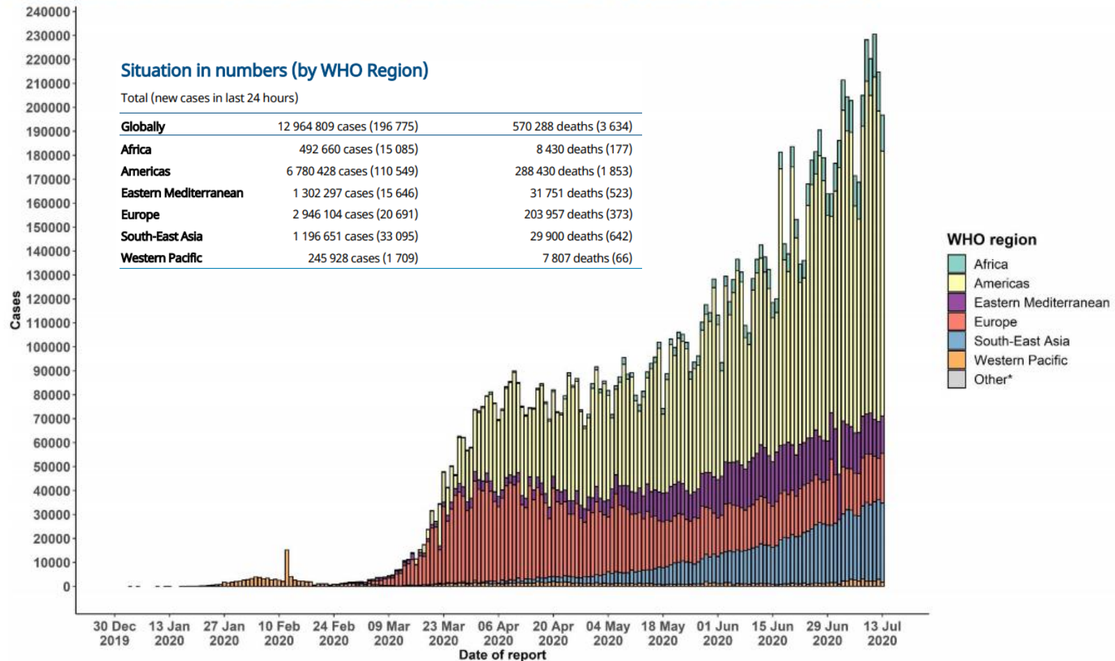
Figure 2. Number of confirmed COVID-19 cases, by date of report and WHO region, 30 December through 14 July**
